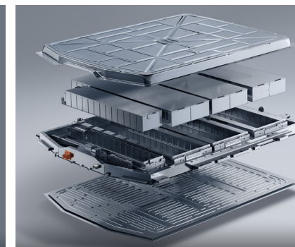
LFP batteries, which offer high safety and long lifespan
